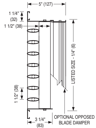
Model 81DH Horizontal Front Blades Double Deflection
