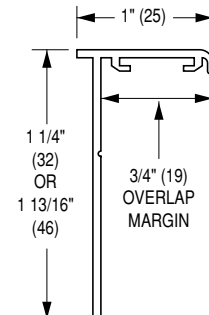
NF Narrow Frame
