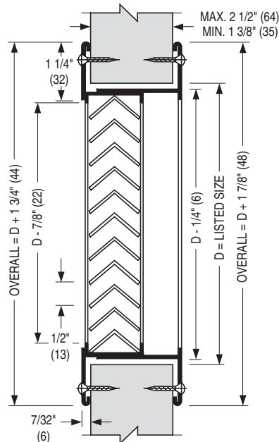
Model 61DGD (Double Flange) Auxiliary Frame Assembly
