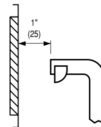
Alnor Velometer with 2220A or 6070P Jet Probe
