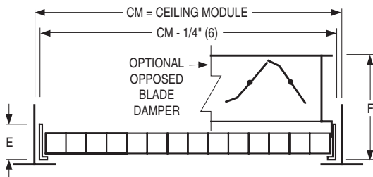
Frame/Border Type L – Lay-in
