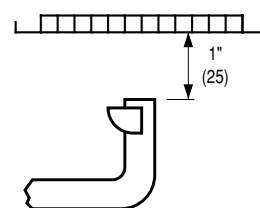
Anor Velometer with 2220A or 6070P Jet Probe
