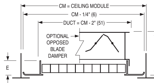
Frame/Border Type S – Surface Mount
