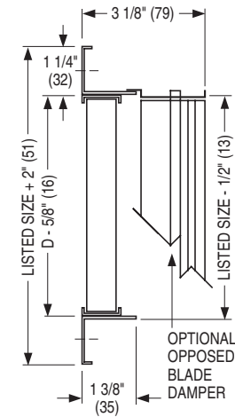
Model 61SV-HD Vertical Blades
