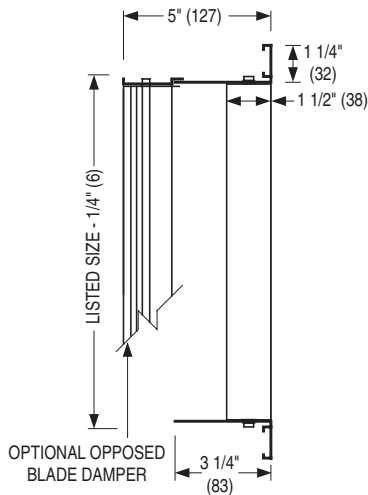
Model 81SV Vertical Blades Single Deflection
