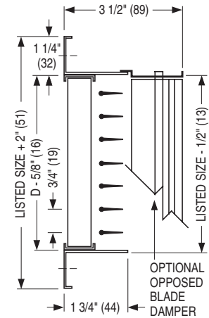
Model 61DV-HD Vertical Blades
