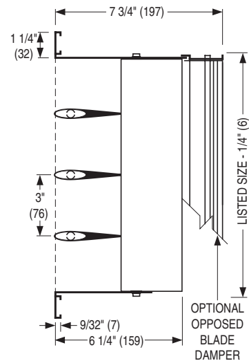
Model 813DH Horizontal Front Blades Double Deflection
